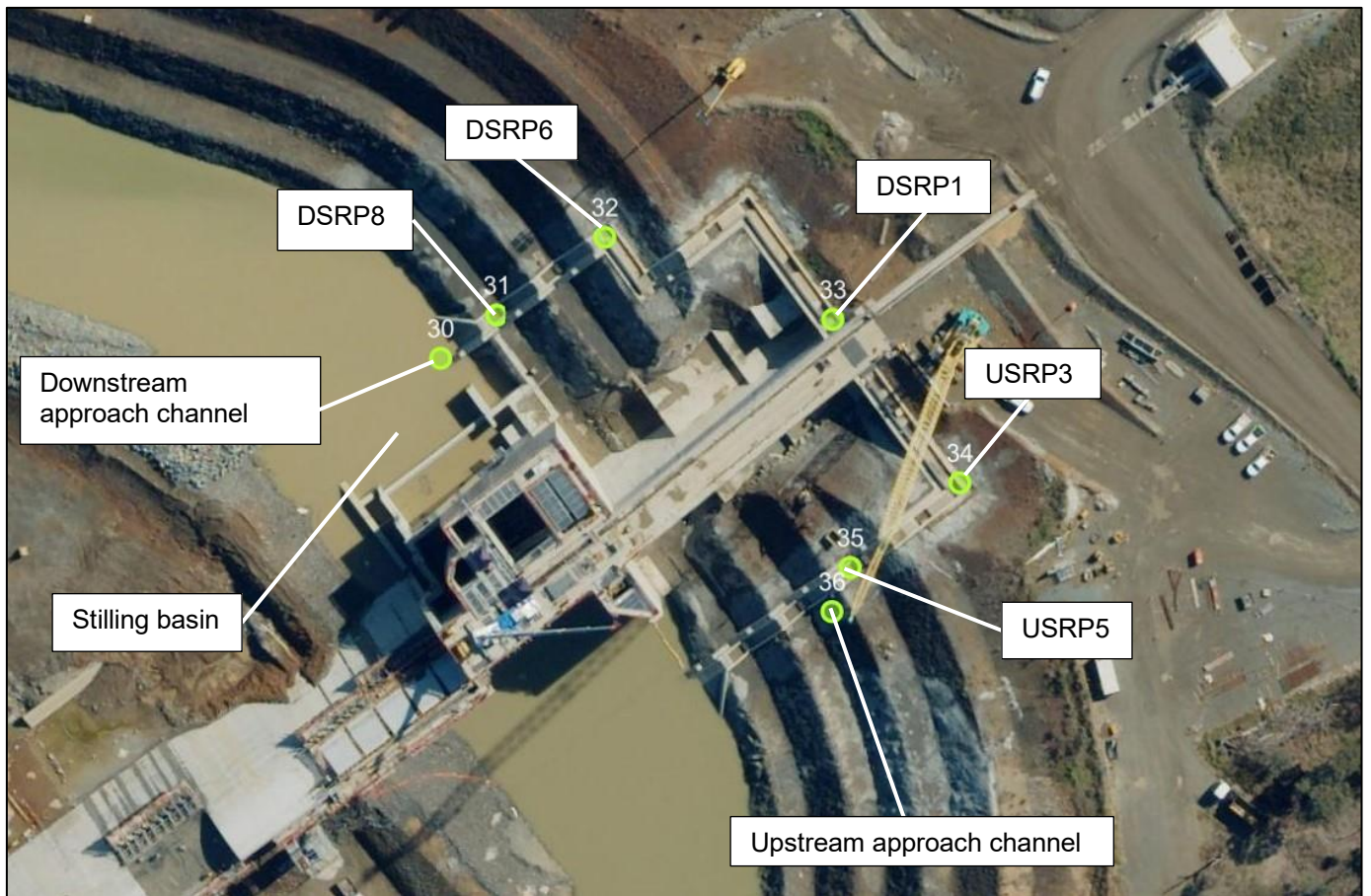
Figure 2.3 Turtle passage monitoring – acoustic hydrophone array (shown as green circles)
