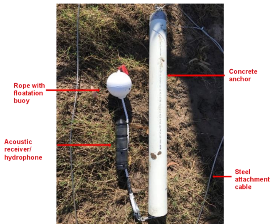
Plate 2.6 Vemco VR2-W underwater acoustic hydrophone mounted to 12 mm rope with floatation buoy and steel attachment cable
