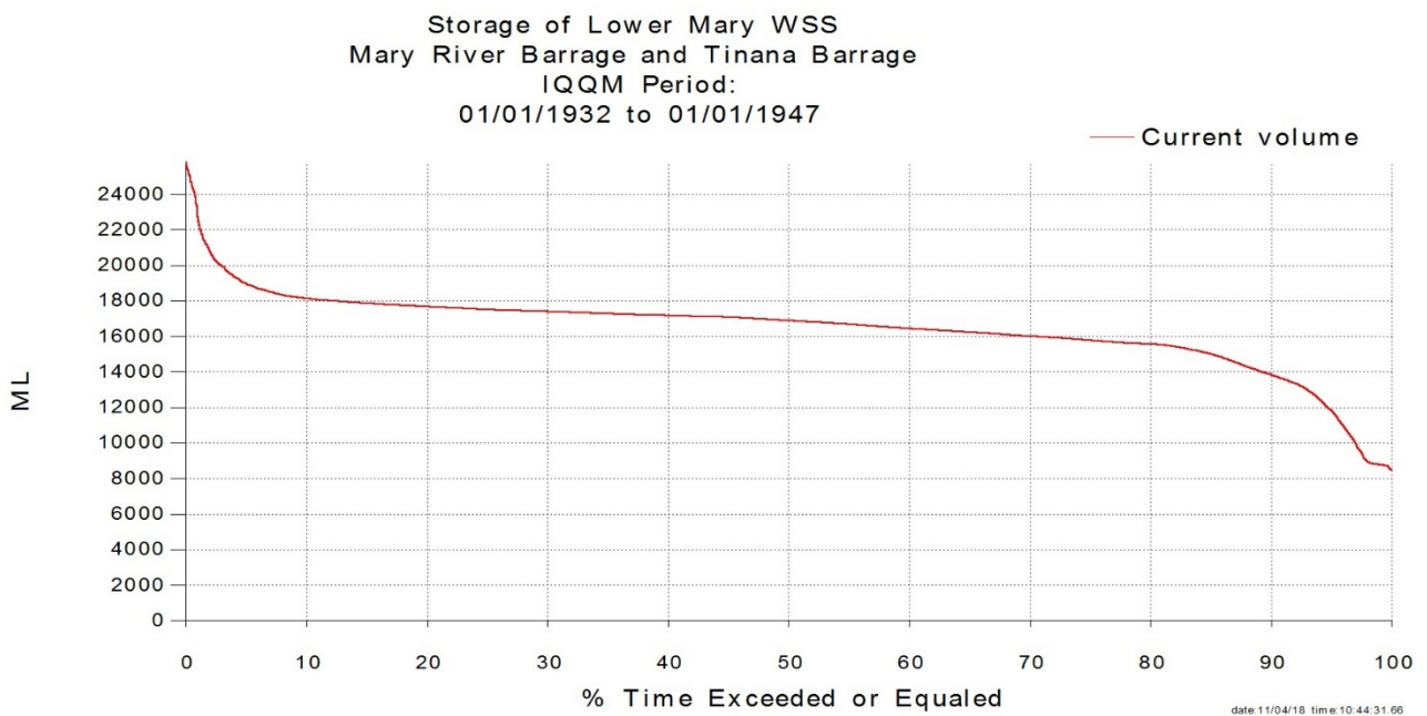
Figure 2.7: Lower Mary River WSS exceedance curve
