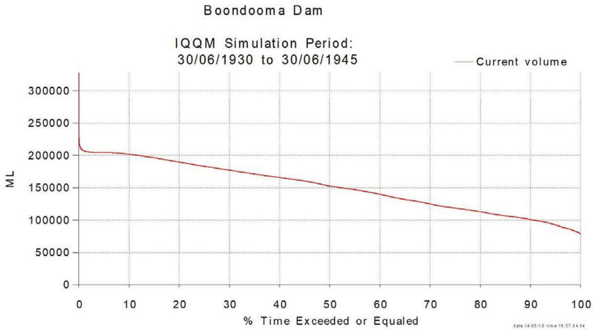
Figure 2.3: Boondooma Dam MPO nom chart
