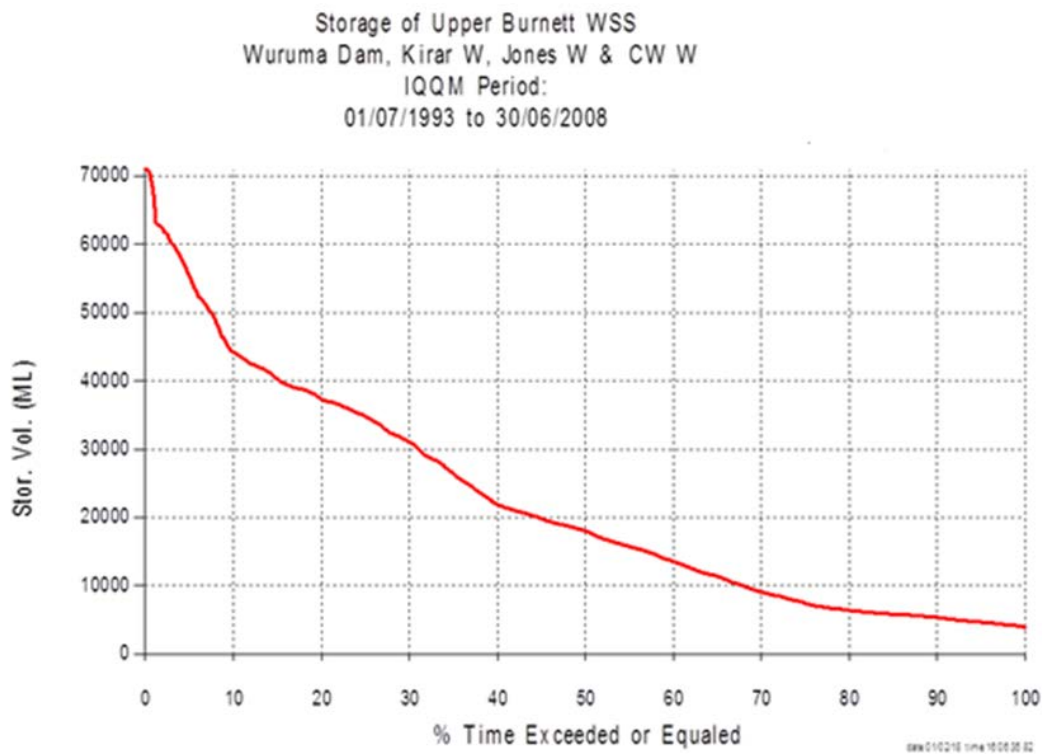
Figure 2.11: Upper Burnett WSS exceedance curve
