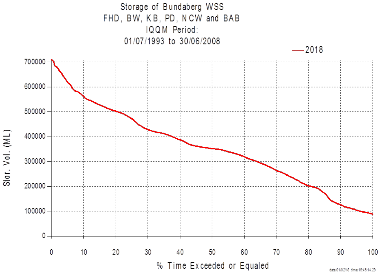
Figure 2.4: Bundaberg WSS exceedance curve
