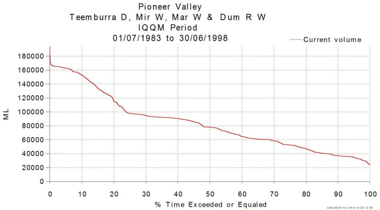
Figure 2.9: Exceedance curve for Pioneer Valley WSS
