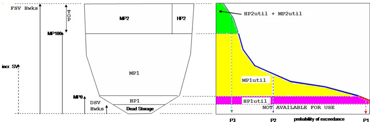
Figure 2.14: Relationship between parameters used in the calculation of Headworks utilisation Factors
