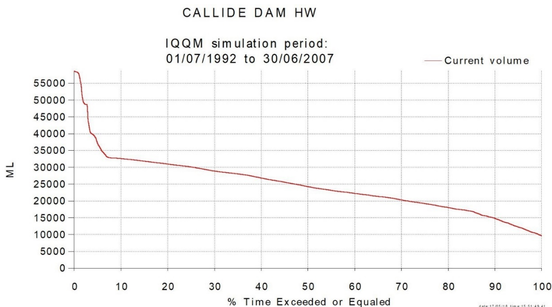
Figure 2.5: Callide Dam exceedance curve
