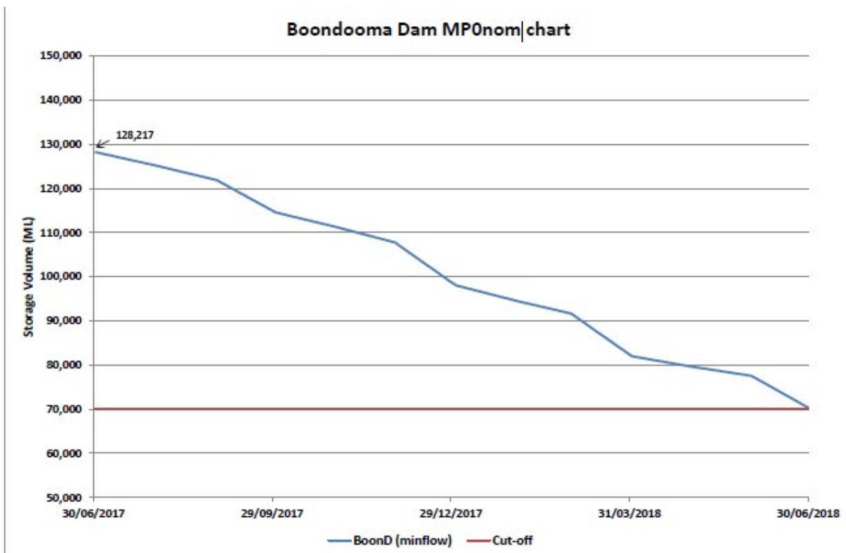
Figure 2.3: Boondooma Dam MPO nom chart
