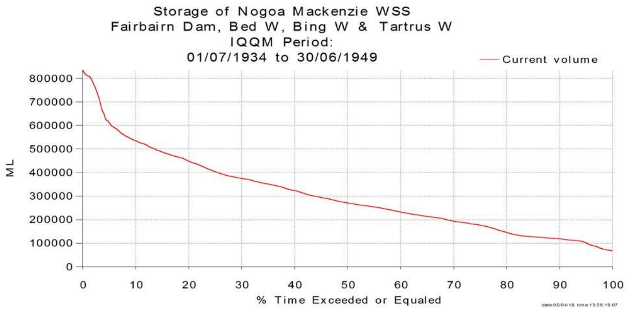
Figure 2.8: Nogoia Mackenzie WSS exceedance curve
