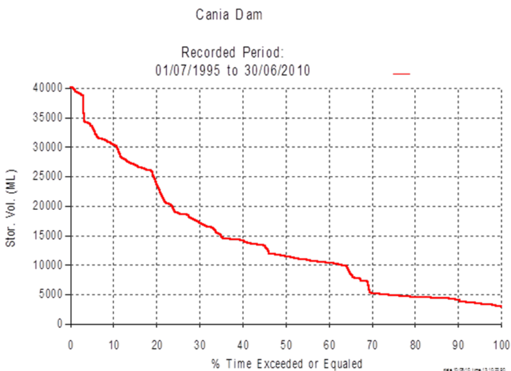
Figure 2.10: Cania Dam exceedance curve
