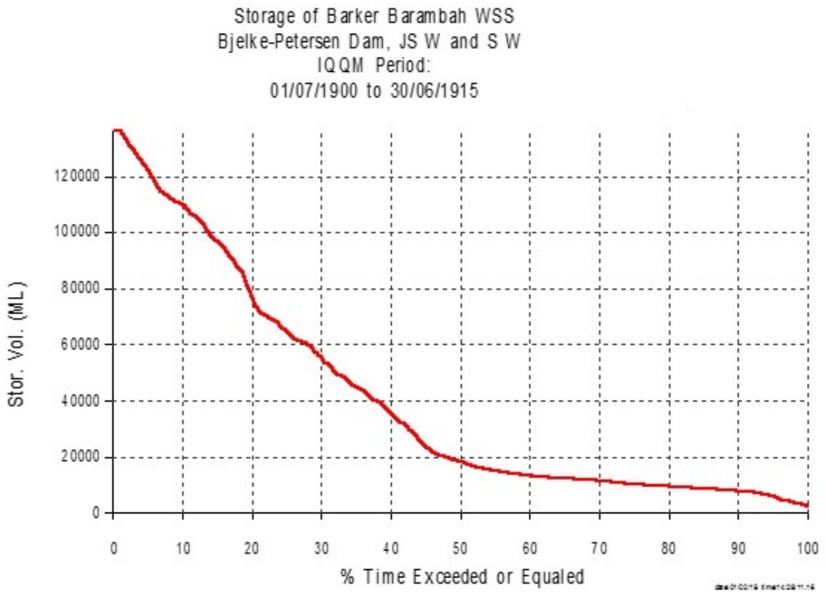
Figure 2.1: Barker Barambah WSS exceedance curve
