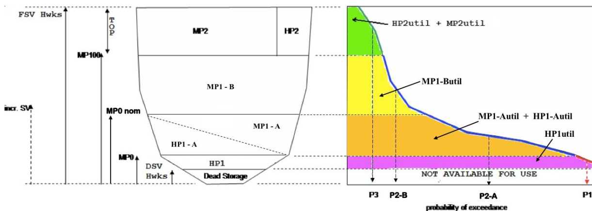
Figure 2.15: Relationship between parameters used in the calculation of Headworks Utilisation Factors for situations where in a 'in-year MP cut-off rule' applies.
