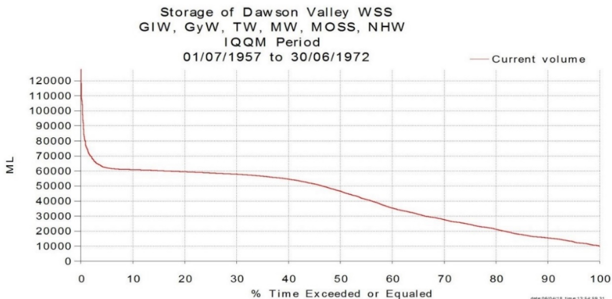
Figure 2.6: Dawson Valley WSS exceedance curve
